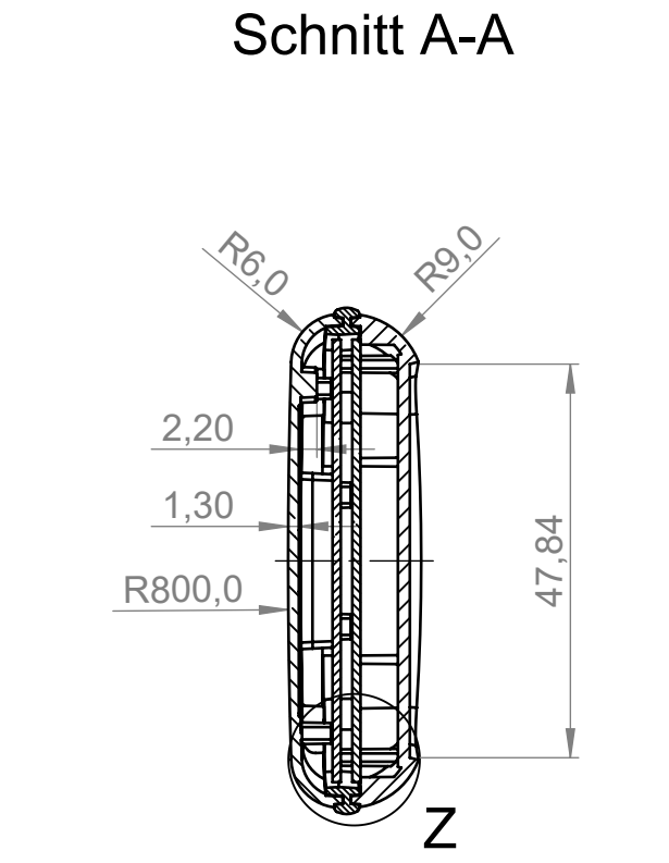
Folientastatur max. 1,20mm dick inkl. Klebefolie Membrane keyboard max. thickness 1,20mm incl. adhesive foil
